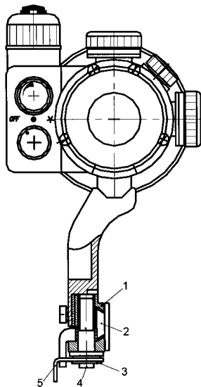
Figure 1 – General view of the sight PN 19K-1-01
