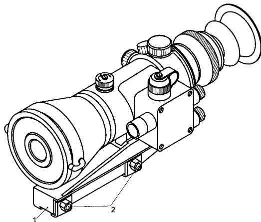
Figure 8 – General view of the sight PN 19K-3-03
