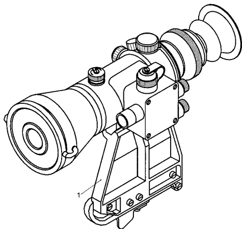
Figure 2 – General view of the sight PN 19K-3-01
